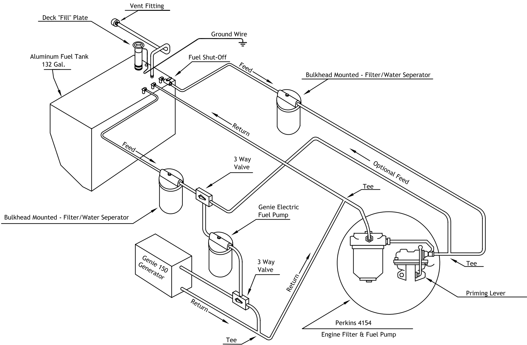
Fuel System For Morgan Out Island 41 Annabelle
